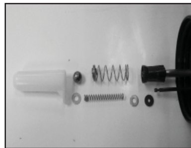
3. Remove and discard pump piston cylinder and associated parts.
